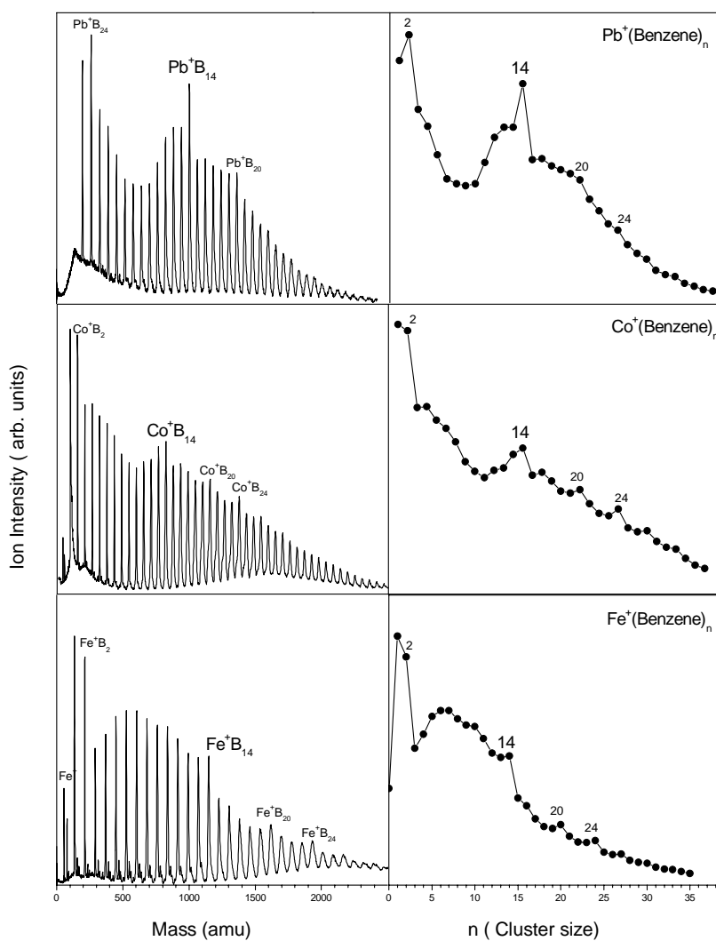
Figure 70: TOF Mass spectra and ion intensity distribution as a function of cluster size of M^+(Benzene)_n where M = Fe, Co and Pb .
