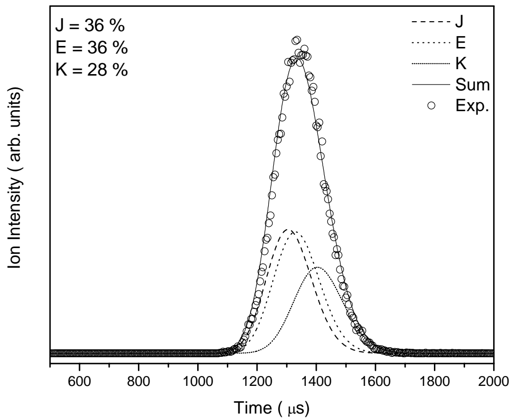
Figure 56: Comparison of the measured ATD of Styrene dimer (\text{C}_8\text{H}_8)_2^+ (circles) drifting in 1.136 Torr He at 303 K ( E/N = 4.38 Td), with the predictions of the transport theory for three structural isomers. These isomers are j (1-phenyltetralin) (dashed line), e (1methyl 3-phenyl indane) (dots) and k (1,3 diphenyl but 1-ene) (short dots).
