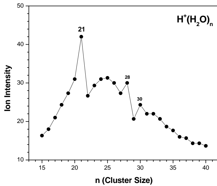
Figure 83: \text{H}^+(\text{H}_2\text{O})_n ion intensity distribution as a function of cluster size
