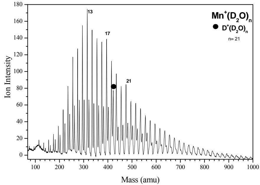
Figure 107: TOF mass spectra of \text{Mn}^+(\text{D}_2\text{O})_n .
