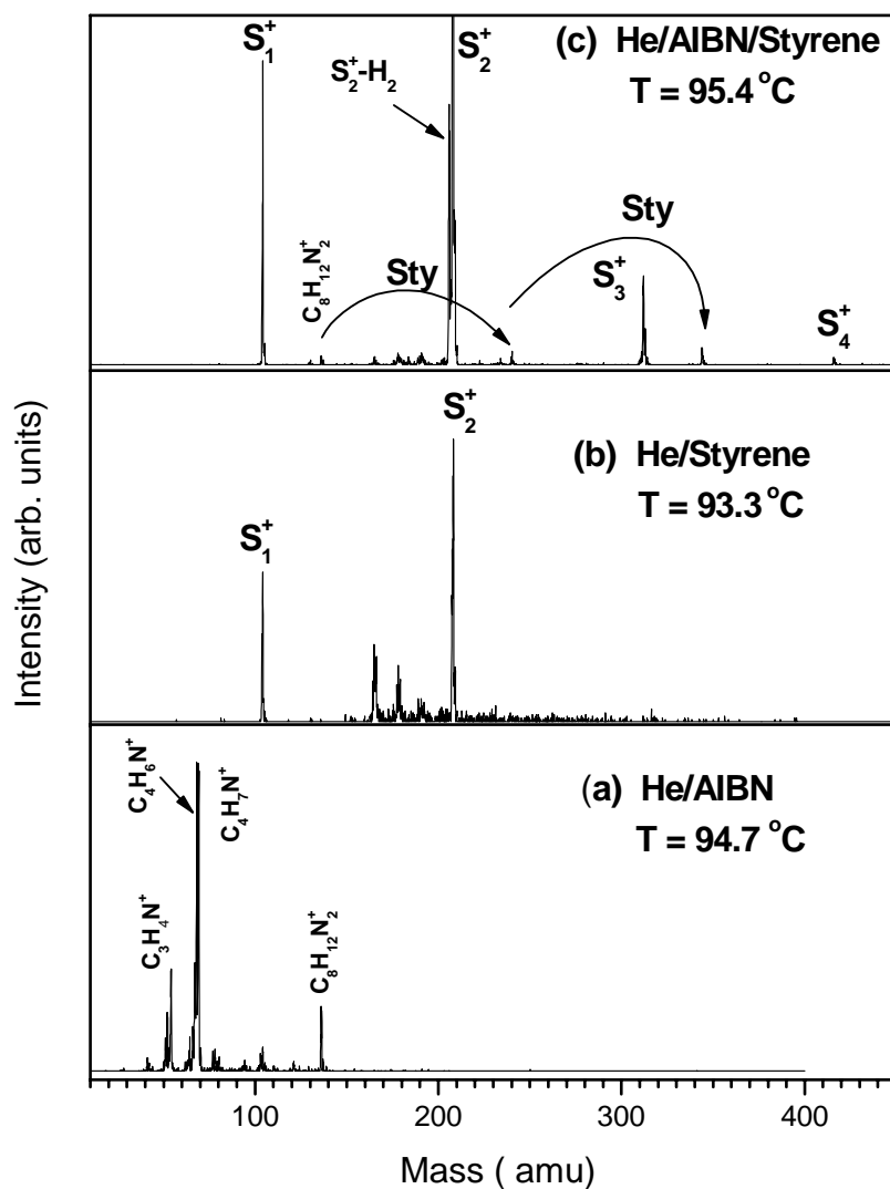
Figure 48: Mass spectra when the source contained: (a) only the initiator AIBN (2,2'-Azo-bis- iso butyronitrile ( \text{C}_8\text{H}_{12}\text{N}_4 ) at T = 94.7\text{ }^{\circ}\text{C} ; (b) only styrene vapor at T = 93.3\text{ }^{\circ}\text{C} and (c) styrene + AIBN at T = 95.4\text{ }^{\circ}\text{C} .
