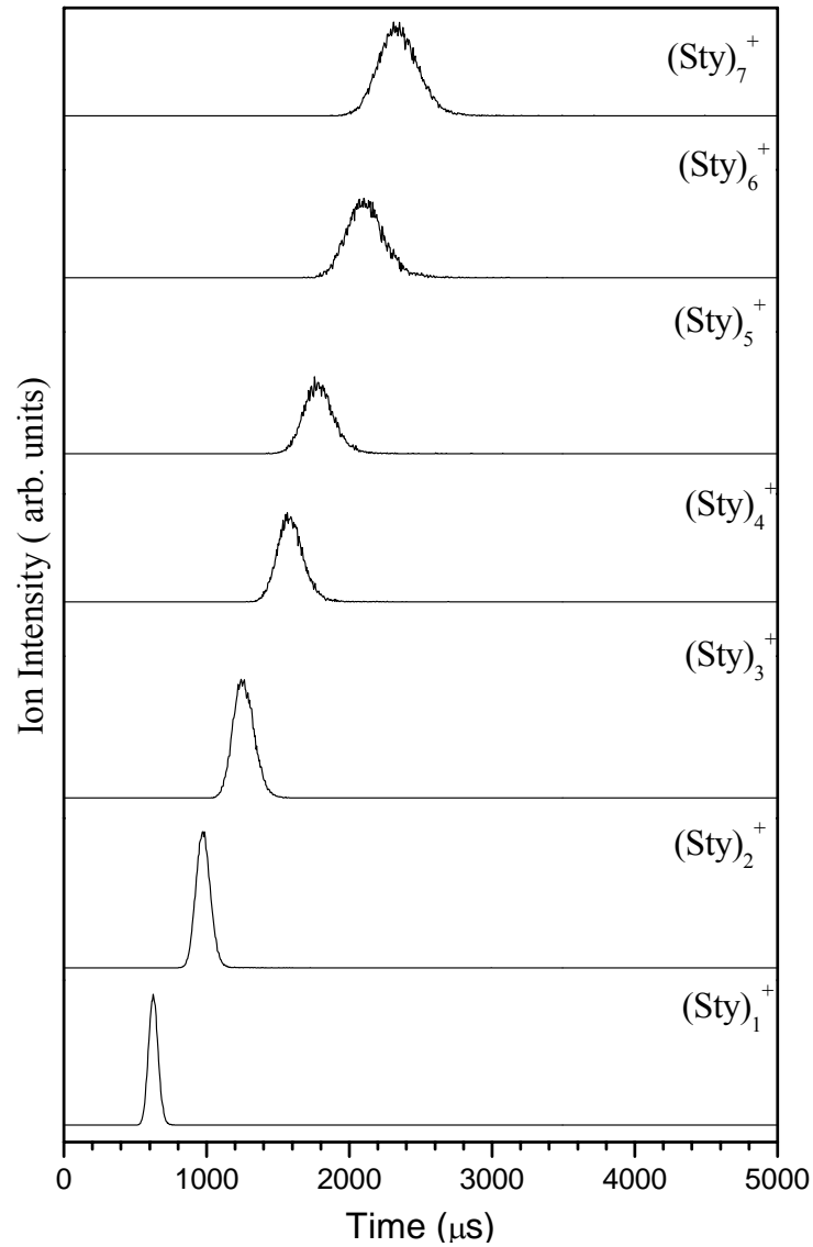
Figure 23 : The measured Arrival time distribution of (\text{C}_8\text{H}_8)_n^+ ions, with n = 1-7 with same E/N = 6.2 \text{ } 3 \text{ } 0.1 .
