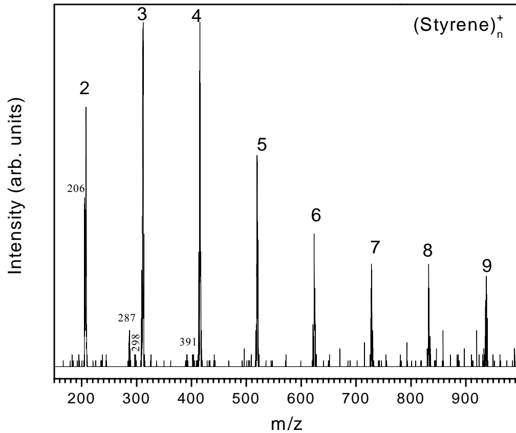
Figure 12: Mass Spectrum of (\text{C}_8\text{H}_8)_n^+ clusters ions produced by 90 eV Electron Impact ionization, and then injected into 1.159 Torr He with 15 eV injection energy.
