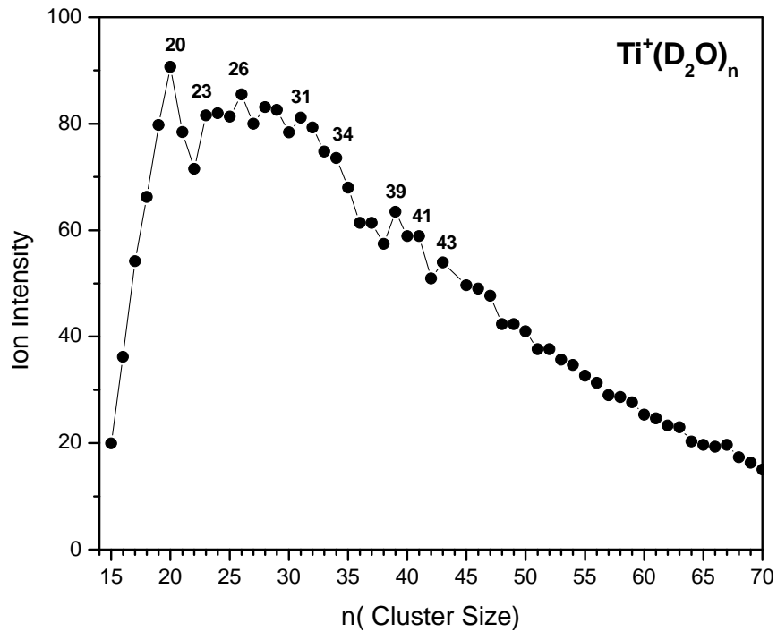
Figure 100: Ti^+(D_2O)_n ion intensity distribution as a function of cluster size.
