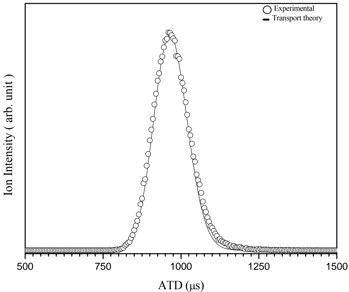
Figure 32: Arrival time distribution of (C_8H_8)_2^+ ions at drift cell temperature of 373 K (circles) and the predicted distribution from transport theory (solid line). Experimental conditions are: 50 \mu s pulse width, injection energy is 15 eV, 1.278 Torr He inside the drift cell, the drift cell temperature is 99.70 ^{\circ}C 18 V voltage difference between the entrance and the exit lenses and E/N = 6.12 Td. The reduced mobility K_0 = 5.34 \text{ cm}^2 \text{V}^{-1} \text{s}^{-1} .
