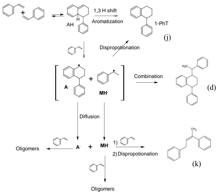
Scheme 9: Proposed mechanism for styrene vapor phase thermal polymerization.
