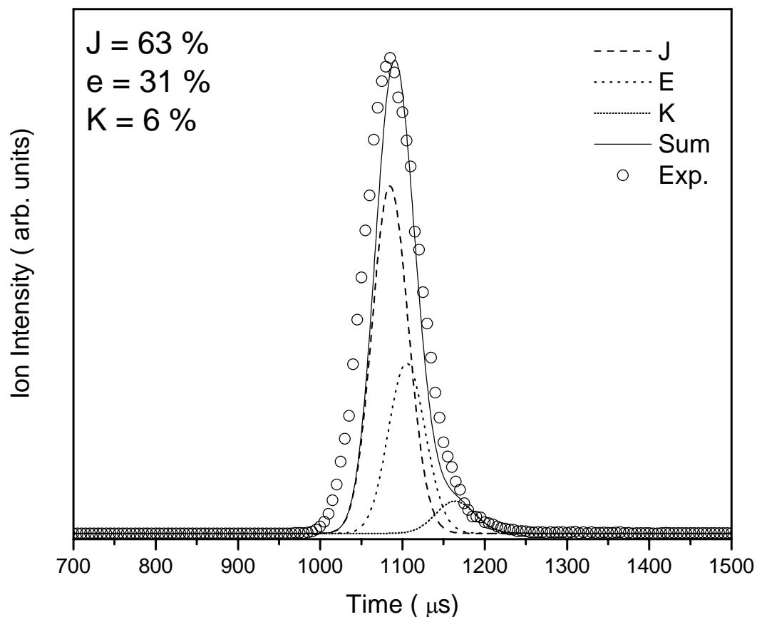
Figure 57: Comparison of the measured ATD of Styrene dimer (C_8H_8)_2^+ (circles) drifting in 1.430 Torr He at 125 K ( E/N = 4.38 Td), with the predictions of the transport theory for three structural isomers. These isomers are j (1-phenyltetralin) (dashed line), e (1-methyl 3-phenyl indane) (dots) and k (1,3-diphenyl but 1-ene) (short dots).
