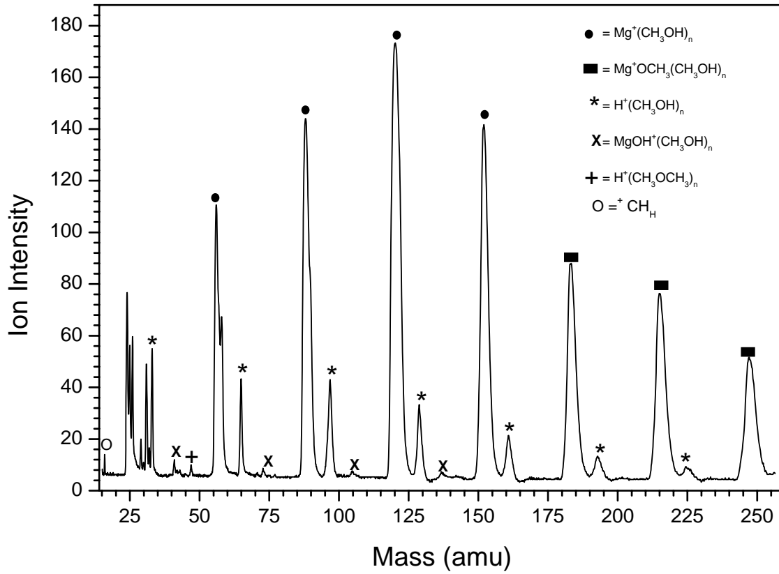
Figure 75: ToF Mass Spectra of \text{Mg}^+(\text{CH}_3\text{OH})_n
