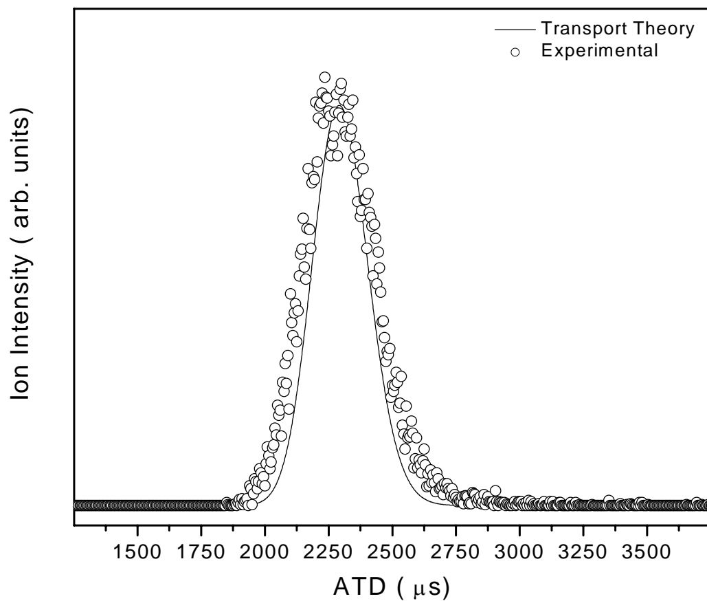
Figure 28: Arrival time distribution of (C_8H_8)_6^+ ions (circles) and the predicted distribution from transport theory (solid line). Experimental conditions are : 50 \mu s pulse width, injection energy is 15 eV, 1.272 Torr He inside the drift cell, the drift cell temperature is 29.9 ^{\circ}C , 20 V voltage difference between the entrance and the exit lenses and E/N = 5.55 Td. The reduced mobility K_0 = 2.79 cm^2V^{-1}s^{-1} .
