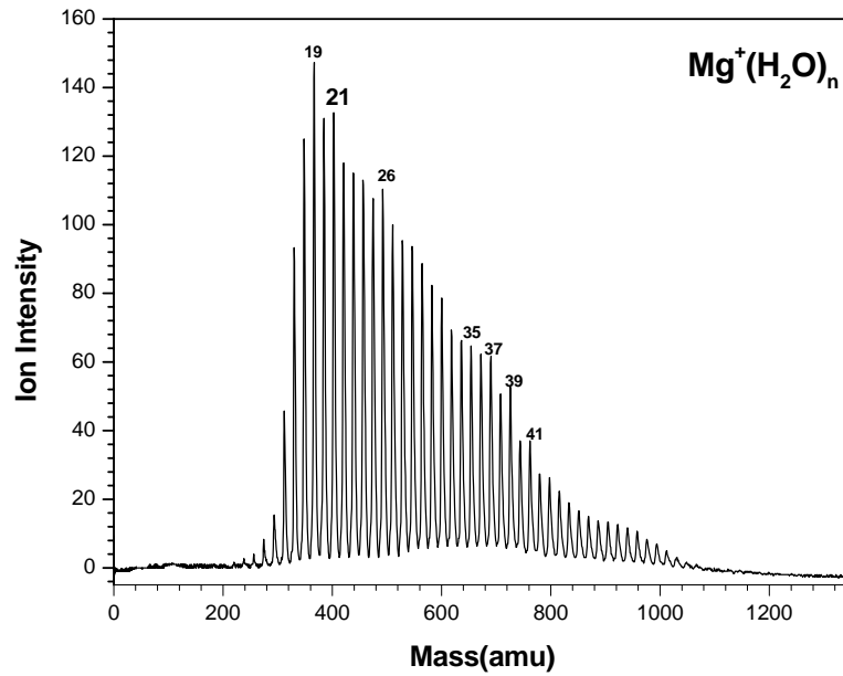
Figure 84: TOF mass spectra of \text{Mg}^+(\text{H}_2\text{O})_n
