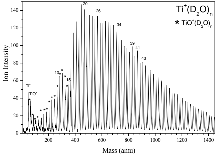
Figure 99: TOF mass spectra of Ti^+(D_2O)_n
