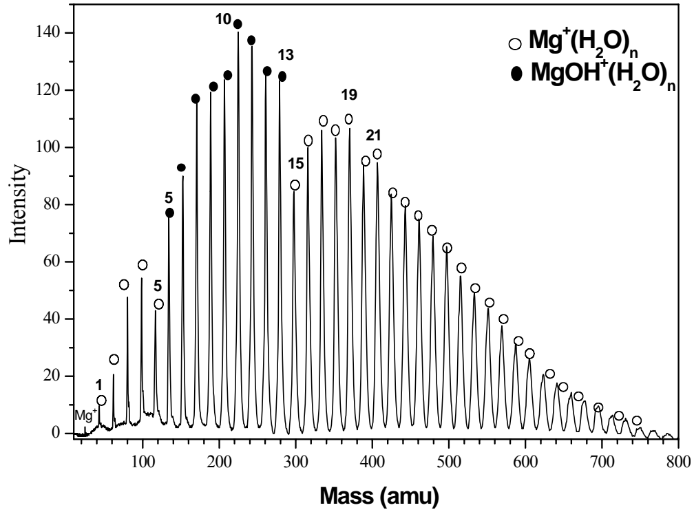
Figure 74: TOF mass spectra of \text{Mg}^+(\text{H}_2\text{O})_n
